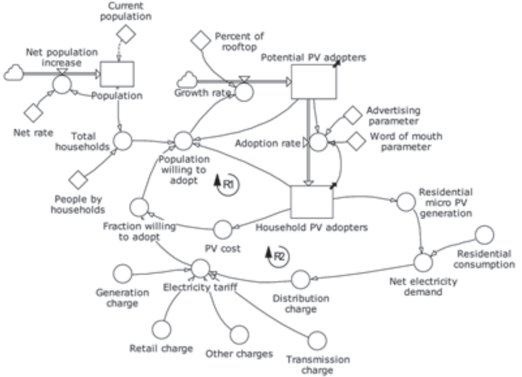
Figure 2. Stocks and flows of the utility death spiral residential sector.
