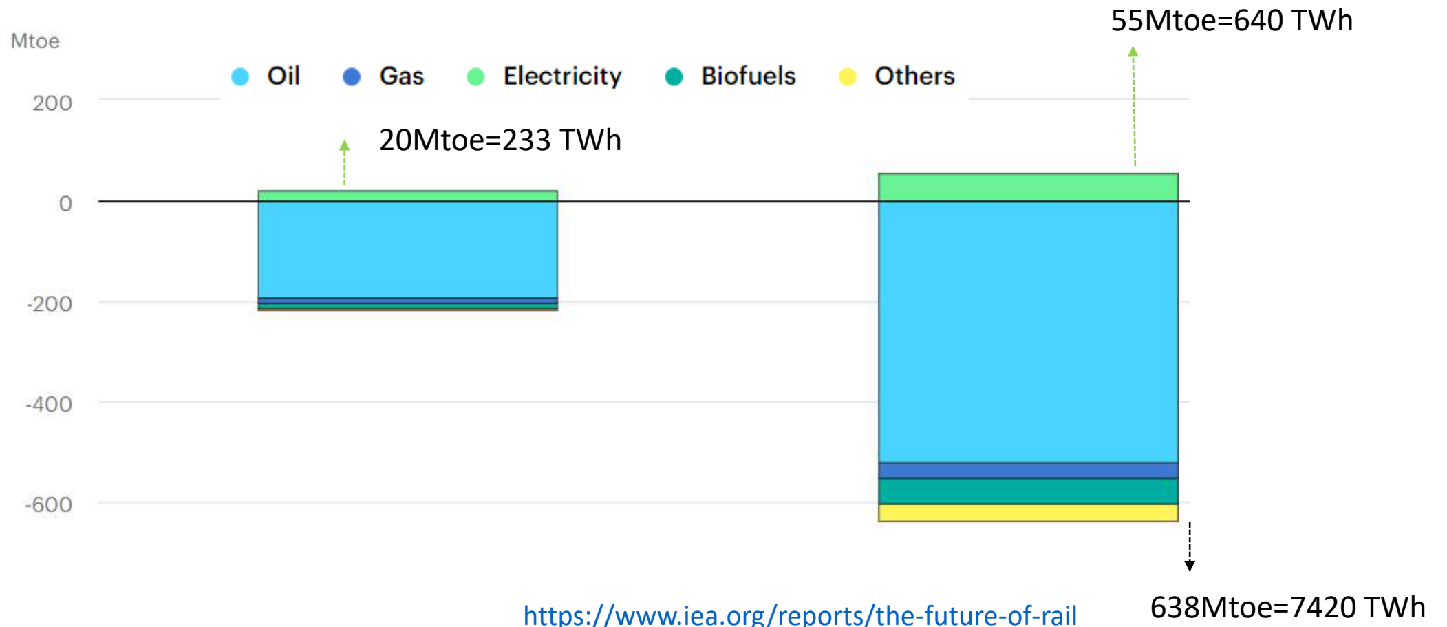
Change in energy demand in the High Rail Scenario relative to a base scenario
